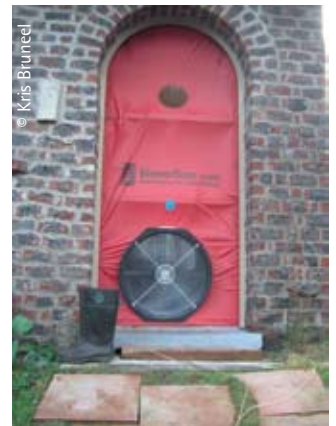
Blower door test: ventilator in deuropening
